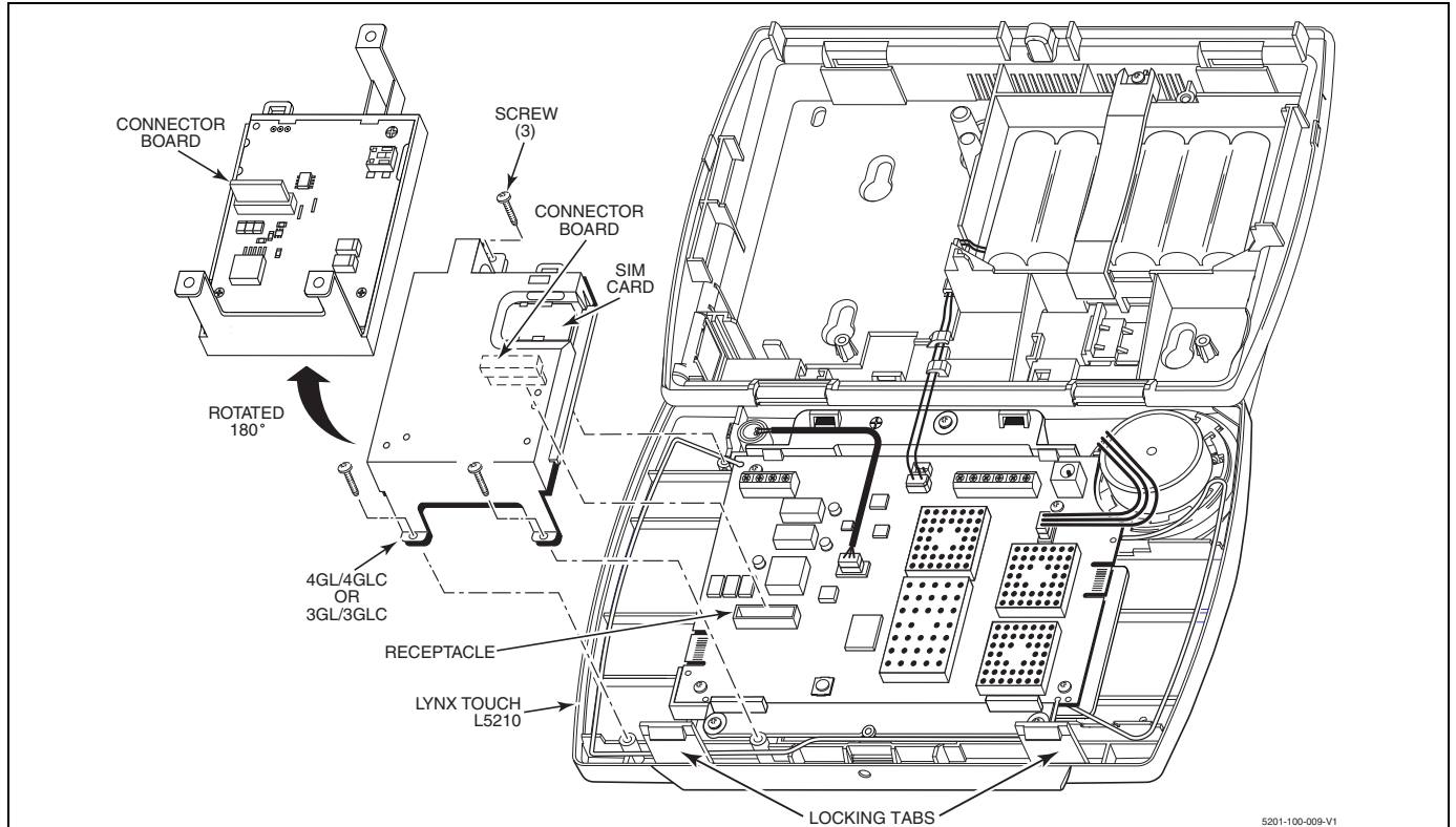
L5210 GSM Communications Installation
